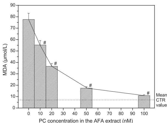
Fig. 4. Dose-dependent inhibitory effect of the AFA extract containing 10–100 nM PC on copper-induced lipid oxidation (TBARS formation) in human plasma samples treated for 2 h at 37°C with 100 μM CuCl 2 . #p < 0.05 from AAPH group.
